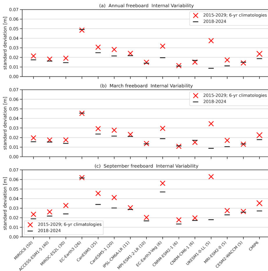
475 Figure 6: Estimates of internal variability (1 ensemble standard deviation, with Bessel correction) of Arctic Ocean total freeboard from ATL20 v4 (processed as discussed in Sect. 2 and 3) for the (a) annual, (b) March and (c) September periods for the 6-year mean over the IS-2 study period 2018-2024 (black lines) and running means across the longer 2015-2029 period (red crosses) for all the CMIP6 models with at least 5 ensemble members. Multi-model CMIP6 mean values shown on the right.
