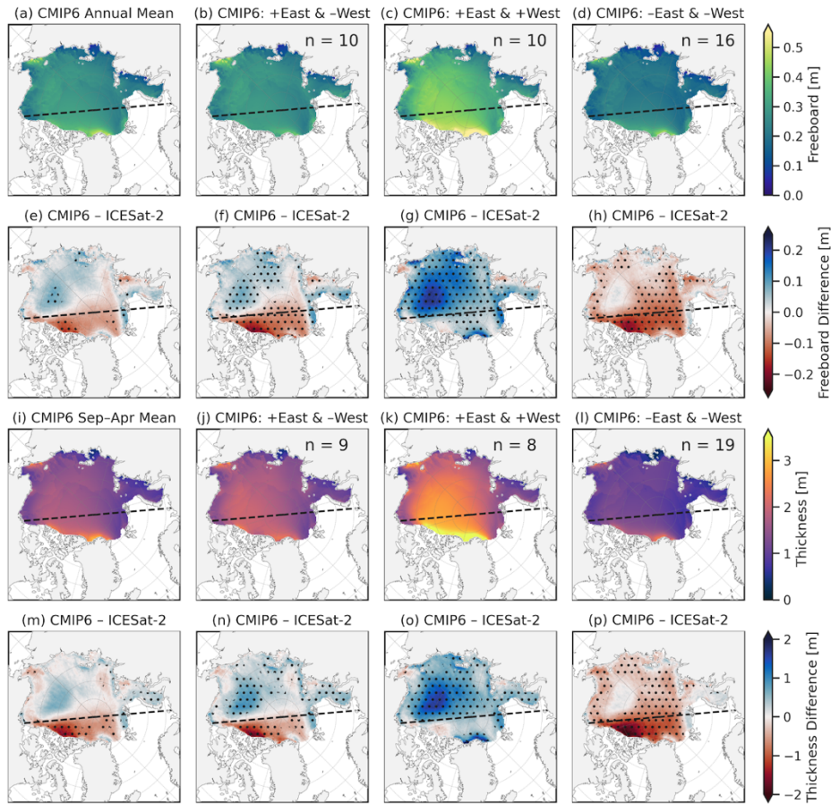
650 Figure 12 (top row) Annual multi-model CMIP6 ensemble mean total freeboard for all models (a) then composites based on their East/West bias pattern (b to d). (second row) top row minus the ATL20 v4 annual mean total freeboards (processed as in Sect. 2 and 3). Third and fourth row show the same but for Sep to Apr Arctic sea ice thickness from CMIP6 and differences with IS2SITMOGR4 v3 thickness data. Stippling indicates where at least 80% of the models in the respective composite agree with the sign of the difference.
