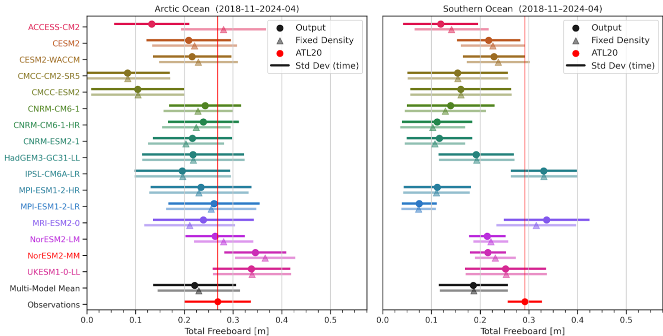
Figure 5: Comparison of mean Arctic Ocean (left) and Southern Ocean (right) total freeboard in the 16-model CMIP6 freeboard subset from the ensemble mean total freeboard output (circles), derived total freeboard assuming a fixed density of 916 Kg m -3 (triangles), and total freeboard observations from ATL20 v4 (processed as discussed in Sect. 2 and 3) (red) for the IS-2 study period (2018-11 to 2024-04). Horizontal lines show the seasonal variability (monthly standard deviation).
