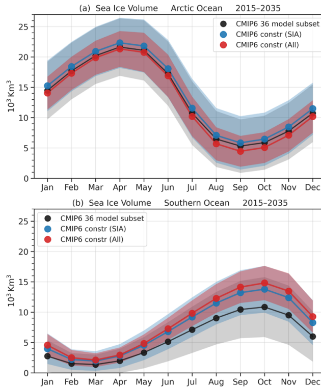
600 Figure 10: Seasonal CMIP6 ensemble mean sea ice volume (lines and circles) and ensemble spread (shading, one standard deviation) from the unconstrained 36-model subset (black), the annual area constrained subset (blue), and the subset constrained with all considered annual variables, including area and freeboard for both hemispheres, and the addition of sea ice thickness for the Arctic only (red).
